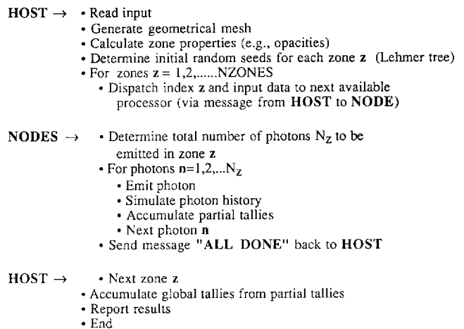
Fig. 6 Dispatching algorithm (local memory)
